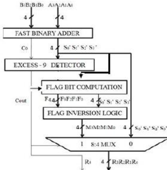
Figure 2 Block diagram of flagged BCD adder
