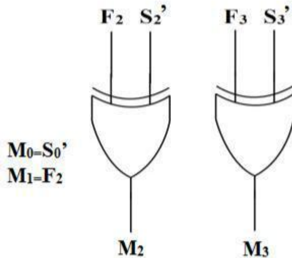
Figure.5 Schematic of flag inversion logic
