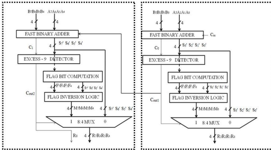
Figure 7 Flagged BCD Adders for 2 Digit Addition
