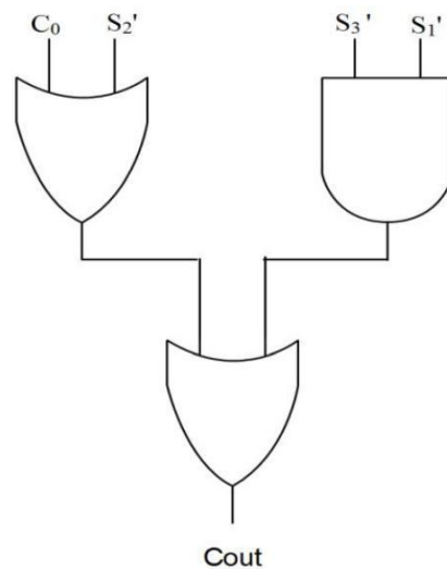
Figure 3. Schematic of Excess-9 detector
